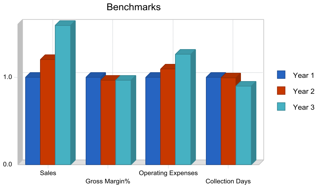
Chart: Benchmarks
